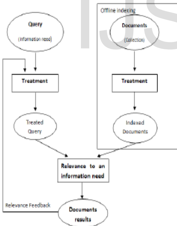
Fig 1.1 Private Information Retrieval Process
